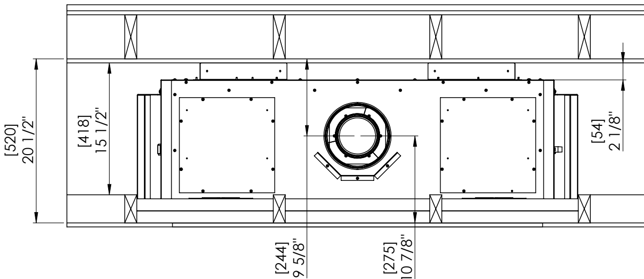
Figure 35(b). Dimension d'un installation vertical
