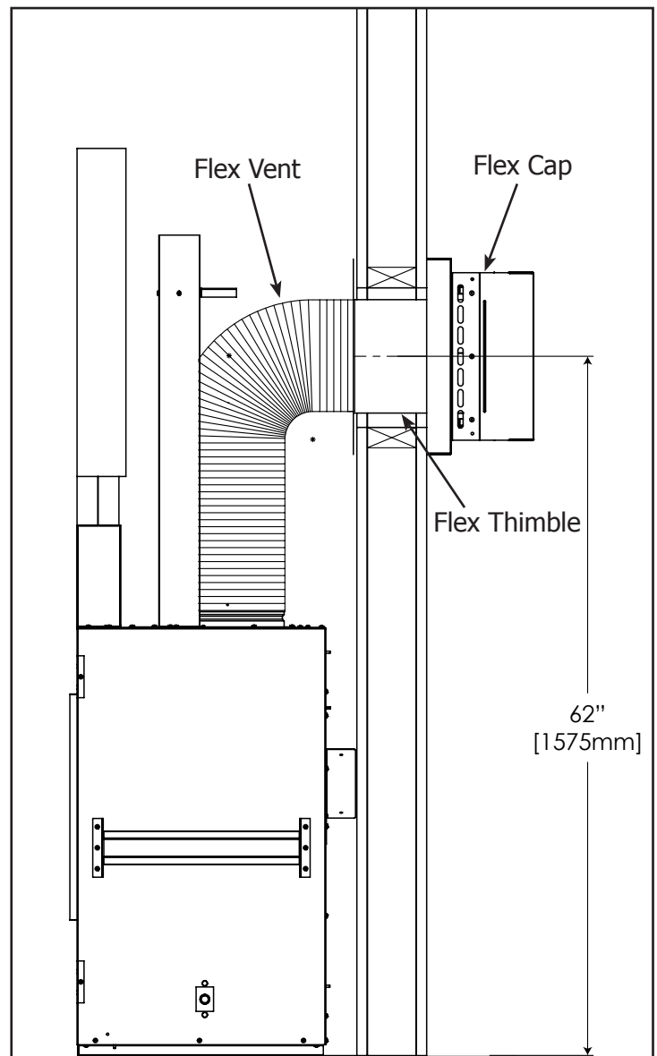
Figure 35. Flex Vent Minimum Install
