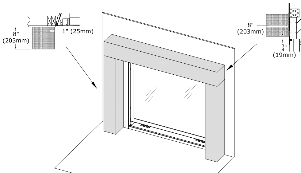
Figure 5.3 - Projections d'un manteau ou contour incombustible - Installation standard
