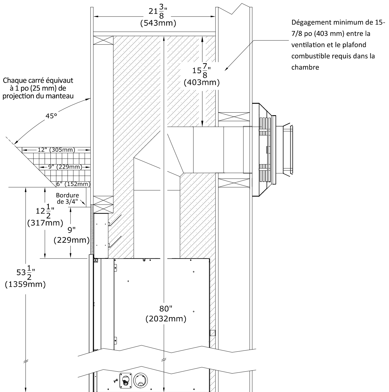
Figure 5.2 - Projections du manteau combustible - Installation standard
