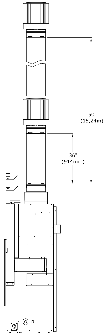
Figure 8.3 - Conduit vertical 4 po x 6-5/8 po
