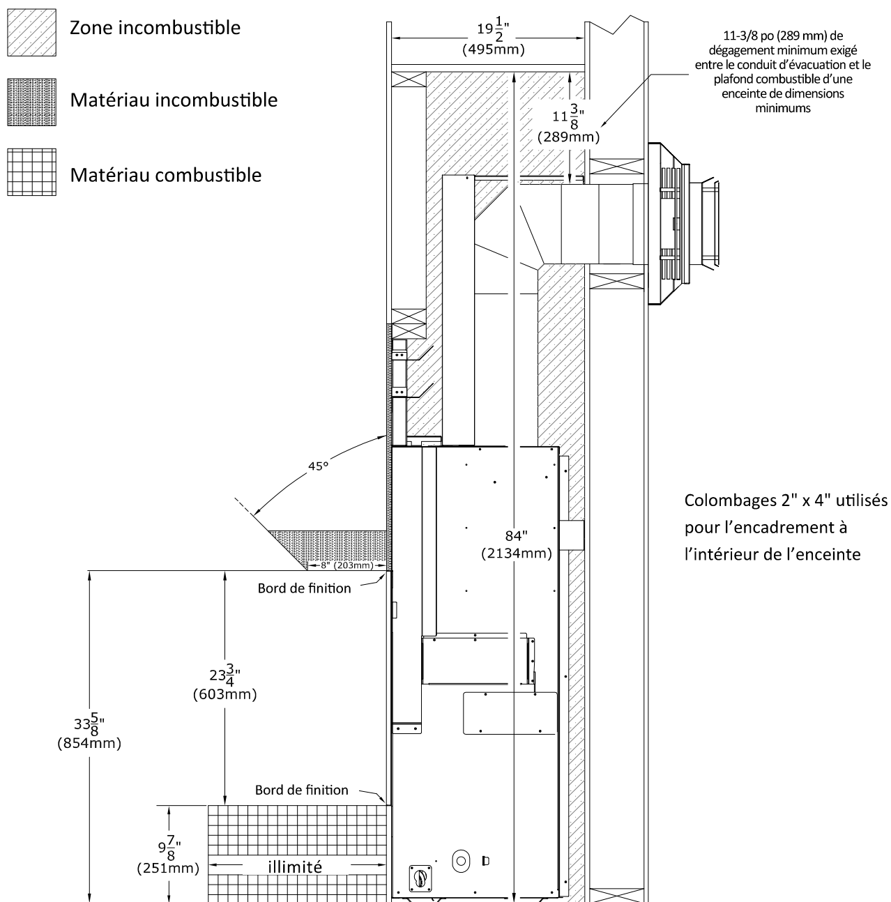
Figure 5.3 - Projections du manteau incombustible - Installation standard
