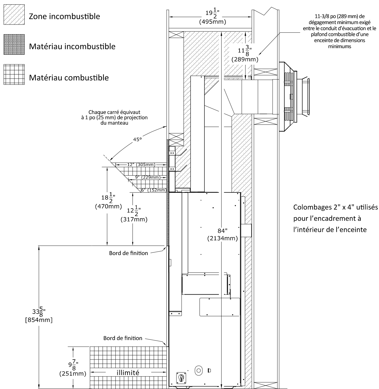
Figure 5.2 - Projections du manteau combustible - Installation standard
