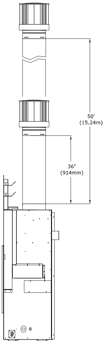
Figure 8.2 - Conduit vertical 4 po x 6-5/8 po
