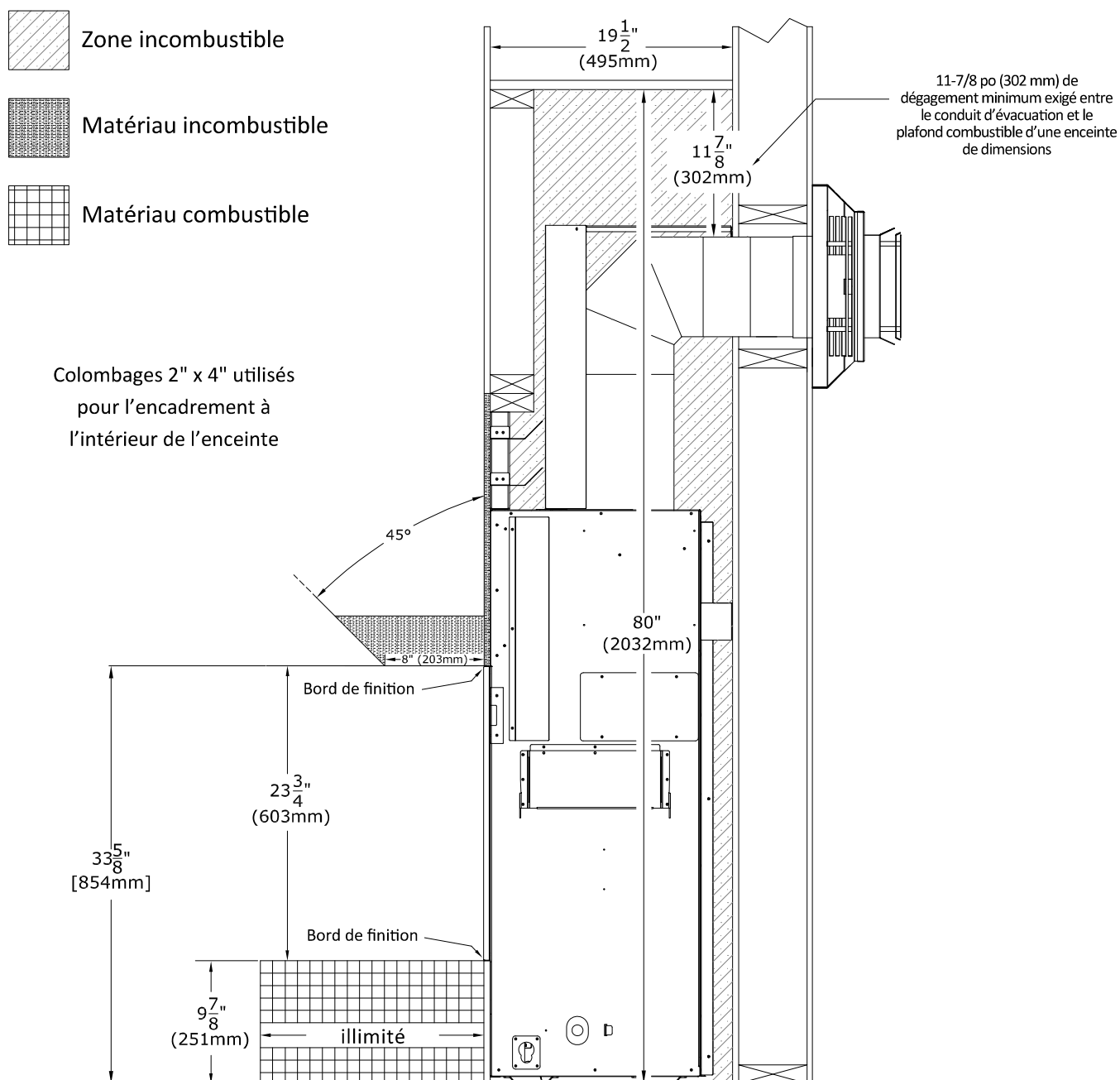
Figure 5.3 - Projections du manteau incombustible - Installation standard
