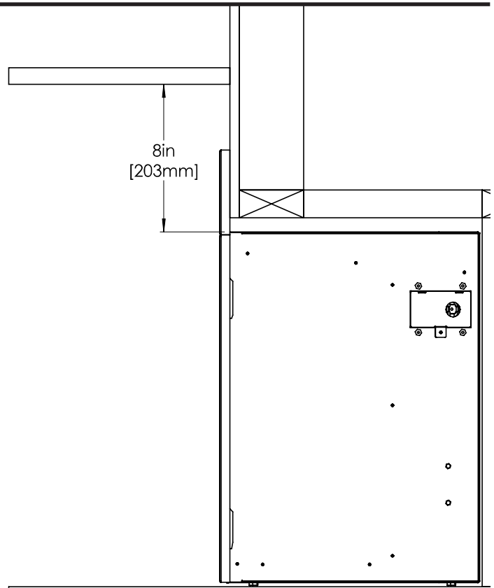
Figure 7: Mantle Clearance
