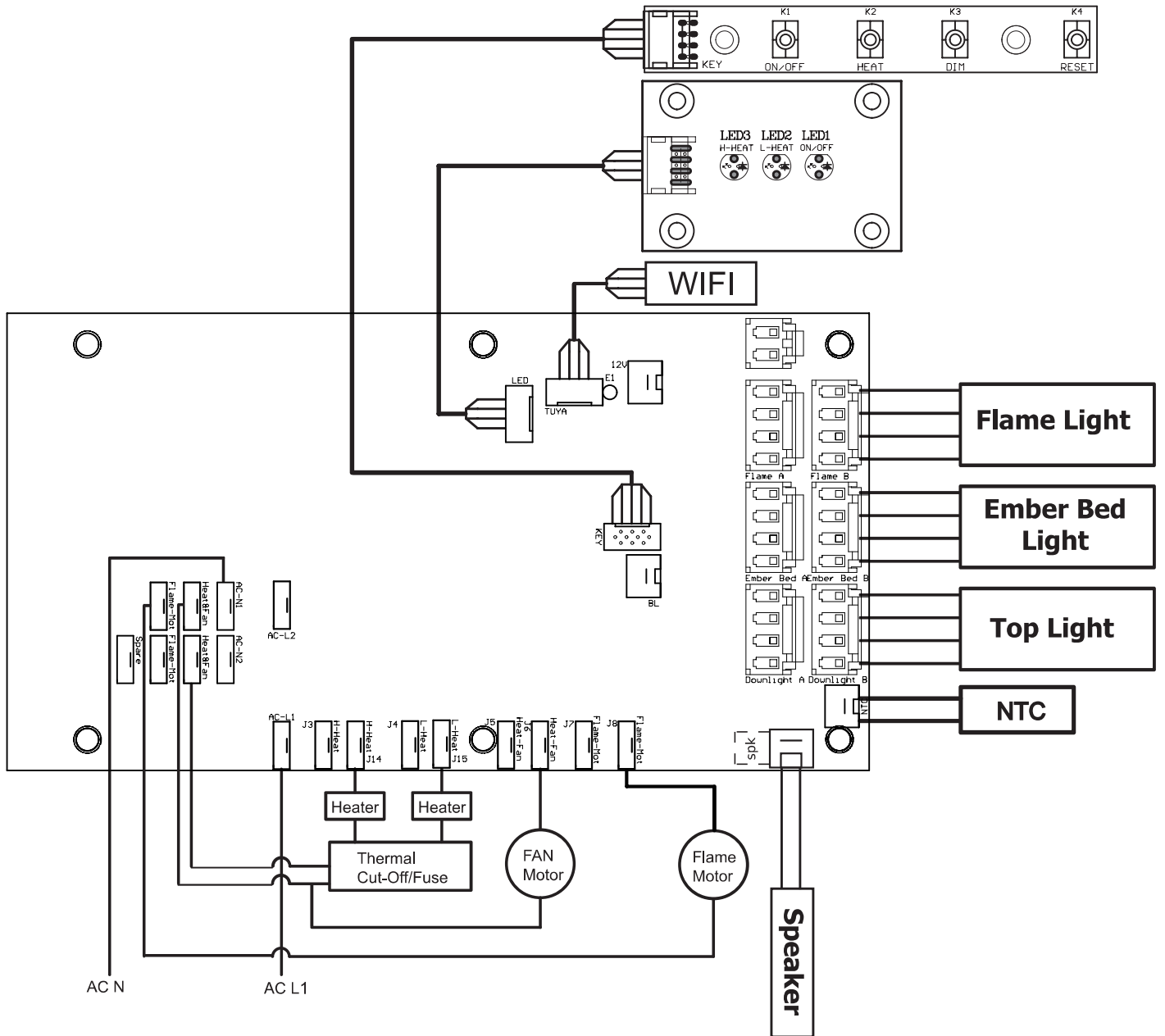
Figure 31: Wiring Diagram
