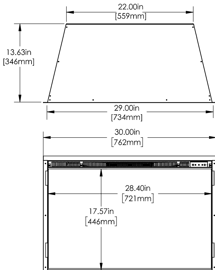
Figure 1: Fireplace Dimensions
