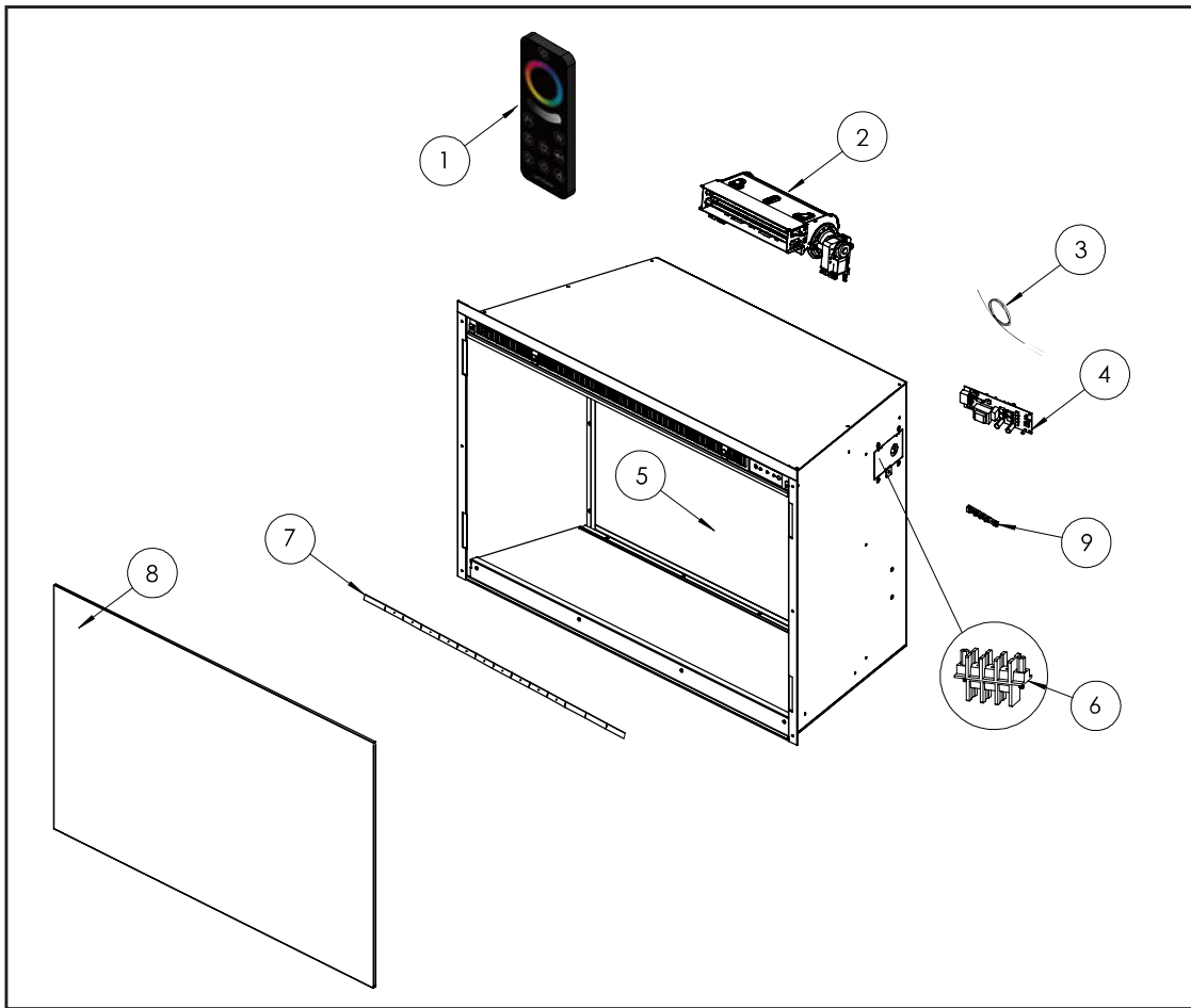
Figure 32: Parts Diagram
