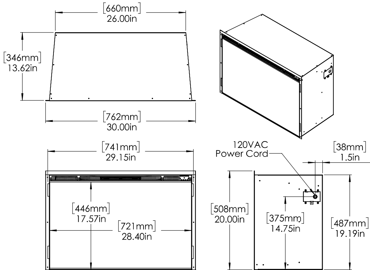
Figure 1: Fireplace Dimensions
