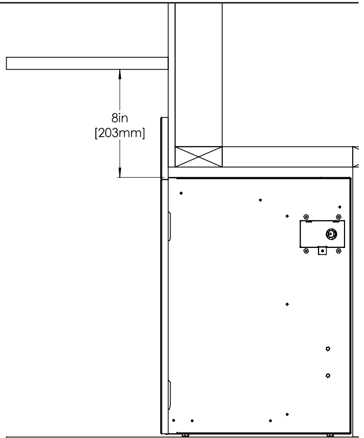
Figure 7: Mantle Clearance
