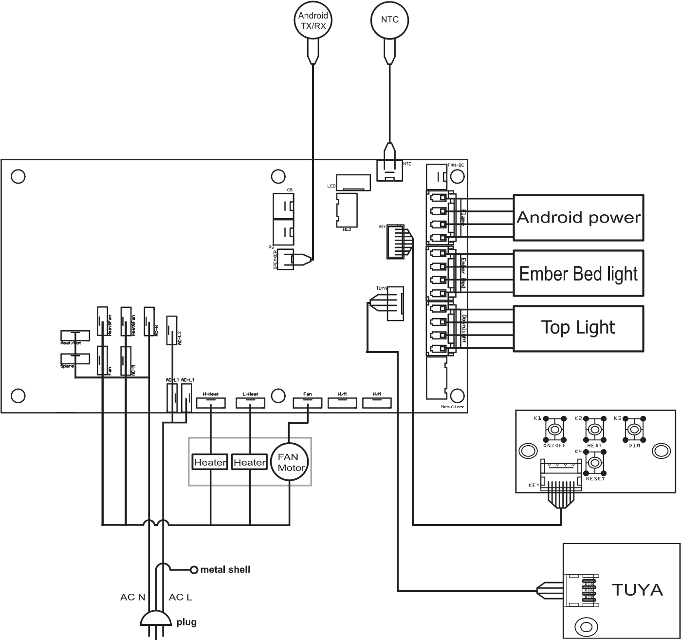
Figure 31: Wiring Diagram
