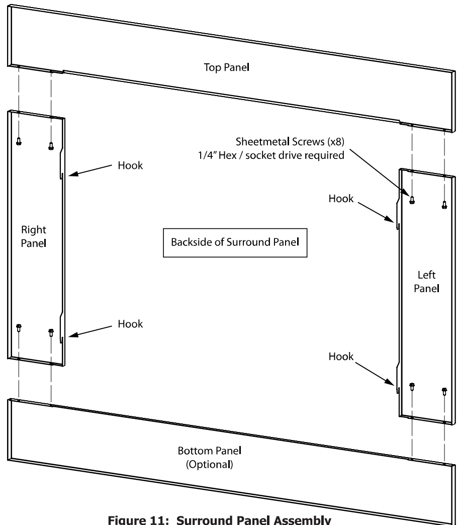
Figure 11: Surround Panel Assembly
