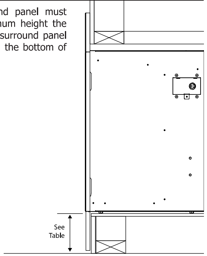
Figure 5: Required Floor Clearance
