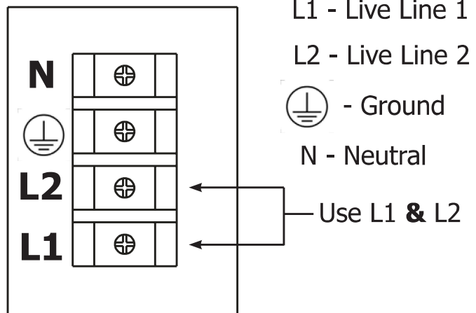
Figure 5: 3000W Wiring Diagram
