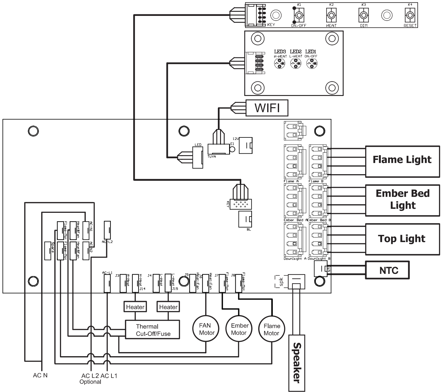
Figure 34: Wiring Diagram
