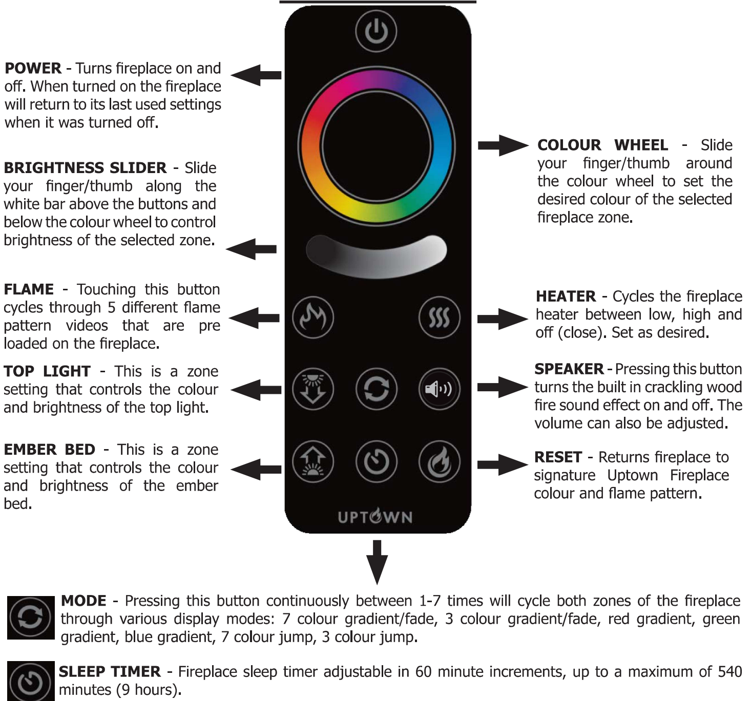
Figure 27: Remote Control
