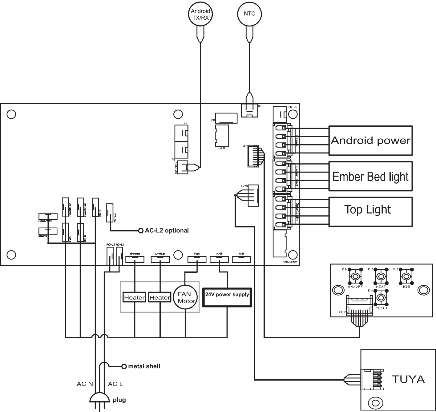
Figure 42: Wiring Diagram
