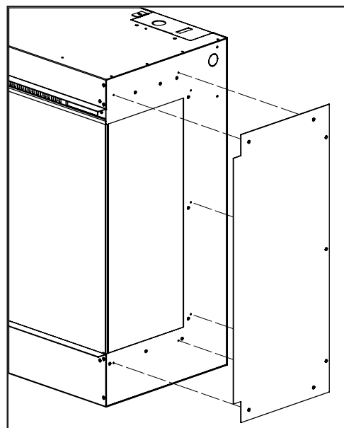
Figure 24: Side Cover Installation
