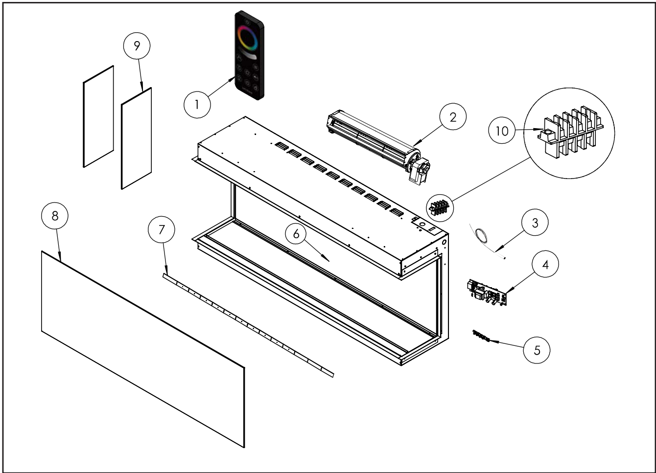
Figure 43: Parts Diagram
