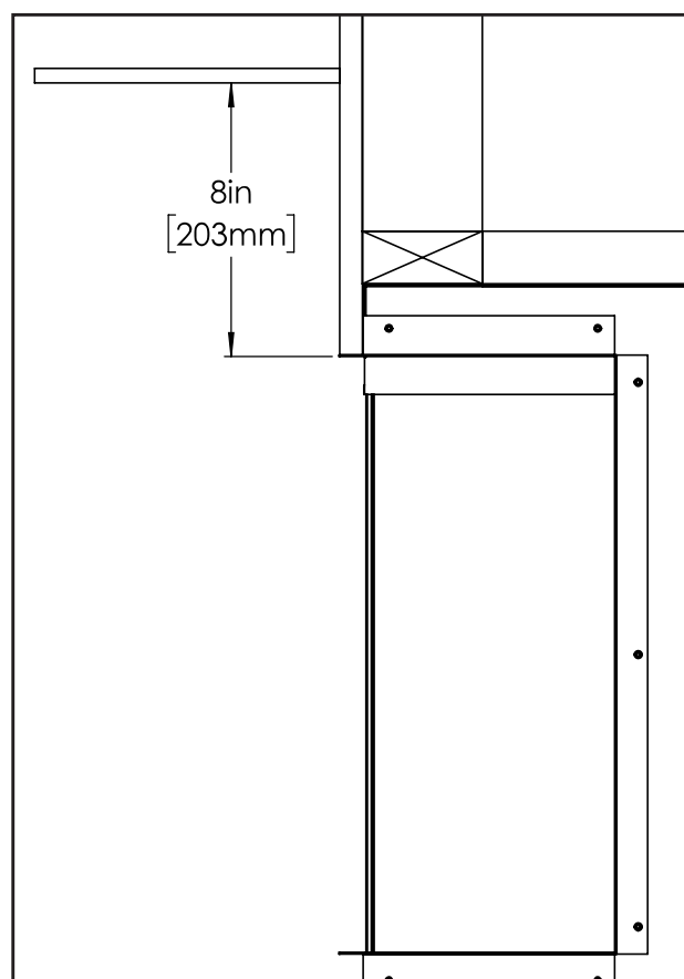
Figure 18: Mantel Clearance
