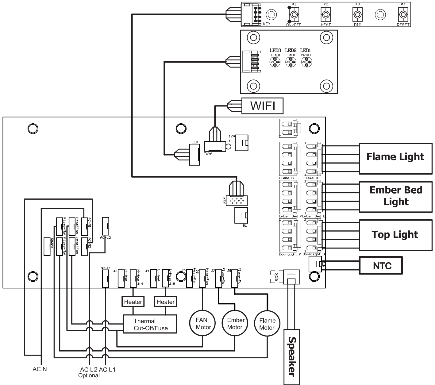
Figure 43: Wiring Diagram
