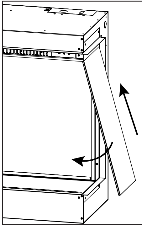
Figure 21: Side Glass - Step 1
