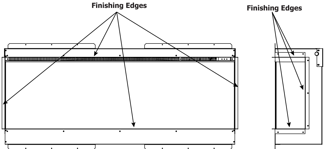
Figure 2: Drywall / Tiling Finishing Edges
